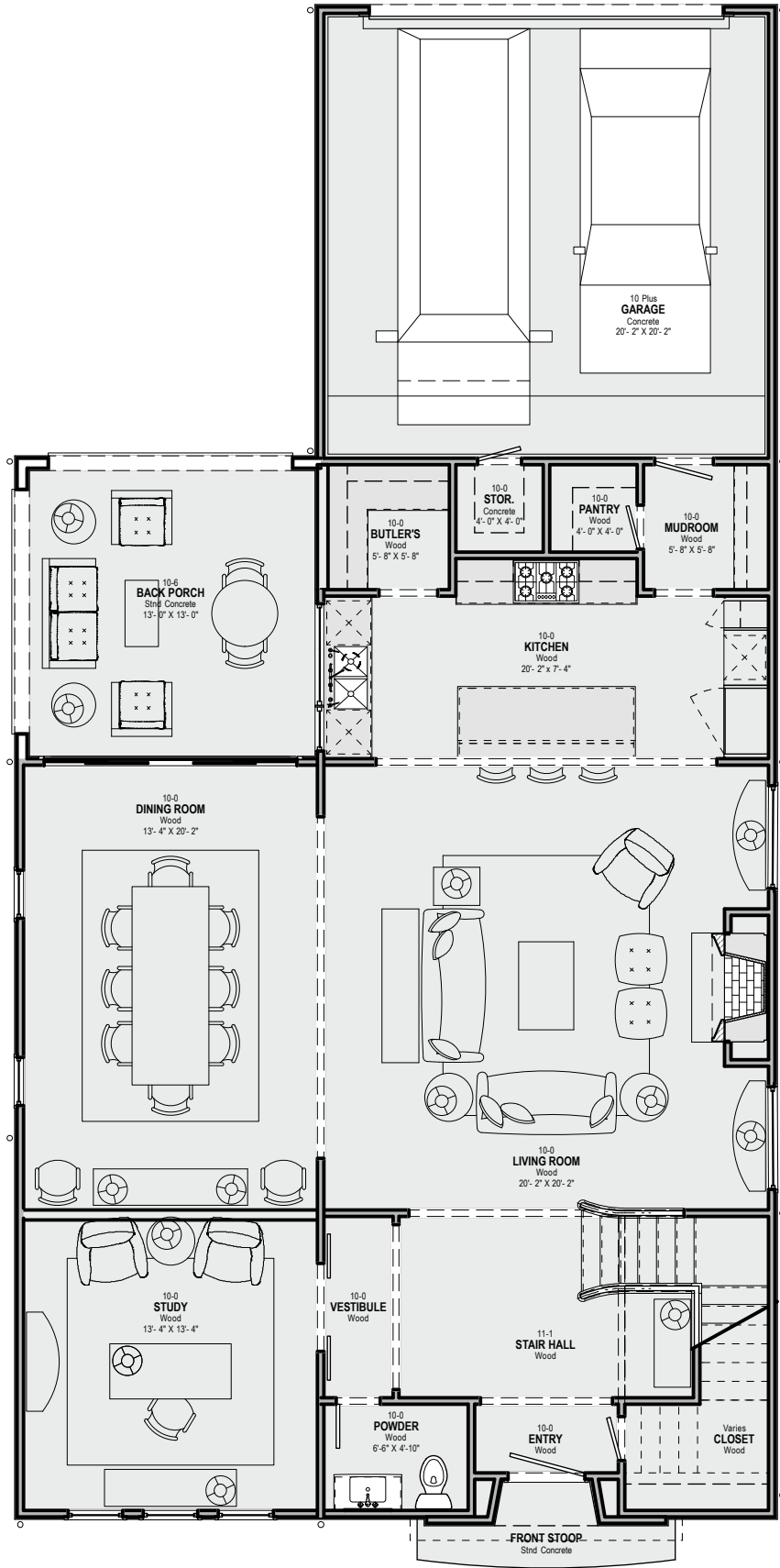
Maravilla Court, A1 Plan (Left) Total Conditioned Area: 3078 sf
